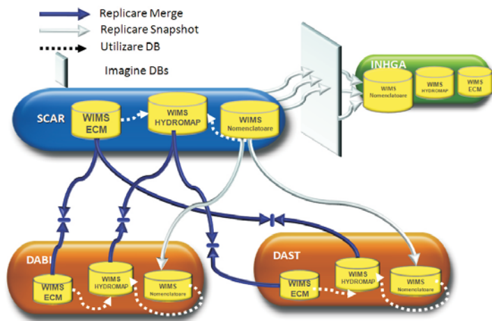
Arhitectura WIMS
